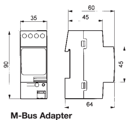
M-Bus Adapter
